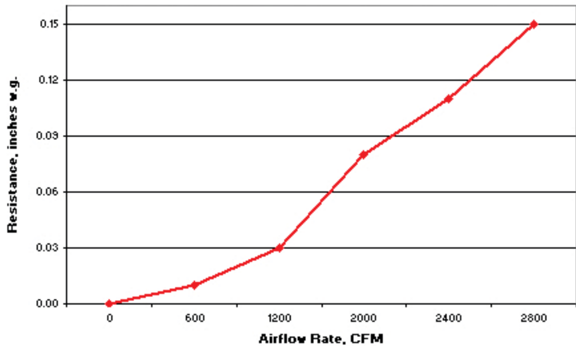
Initial Resistance vs Airflow Rate to 2800 CFM Natural Fiber Filter 24" x 24"
